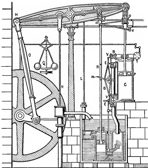
Form of Watt's Engine in 1784
